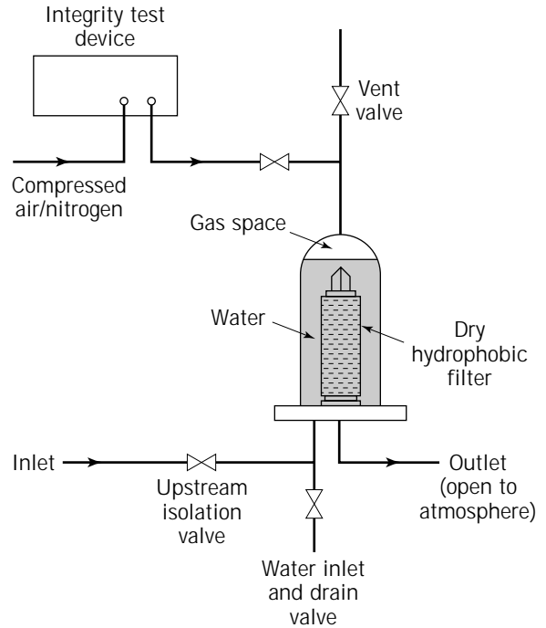
Figure 14. Water intrusion test. Courtesy of Pall Corporation (33).
