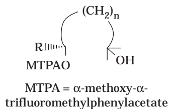
Scheme 4. Determination of enantiomeric excesses of lactones.
