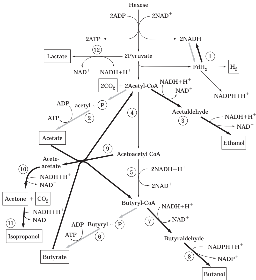
Figure 2. The butanol fermentations. Numbers indicate enzymes as follows: 1, three enzymes that exchange electrons with reduced ferredoxin ( \text{FdH}_2 ), \text{NAD}^+ : and \text{NADP}^+ : ferredoxin oxidoreductases, and hydrogenase; 2, phosphotransacetylase and acetate kinase; 3, acetaldehyde dehydrogenase and ethanol dehydrogenase; 4, acetyl CoA acetyltransferase (or thiolase); 5, three enzymes producing butyryl CoA; 6, phosphotransbutyrylase and butyrate kinase; 7, butyraldehyde dehydrogenase; 8, butanol dehydrogenase; 9, acetoacetyl CoA: acyl CoA transferase; 10, acetoacetate decarboxylase; 11, isopropanol dehydrogenase; 12, lactate dehydrogenase. Thick gray arrows indicate reactions that predominate during acidogenesis; thick black arrows indicate reactions that predominate during solventogenesis. Source: Reproduced with permission from Ref. 25, p. 26.
