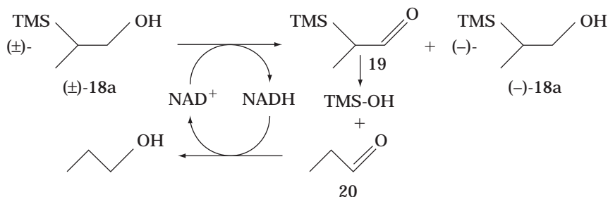
Figure 7. Horse liver alcohol dehydrogenase-catalyzed enantioselective dehydrogenation of 2-trimethylsilyl-1-propanol with in situ coenzyme regeneration. TMS, trimethylsilyl.
