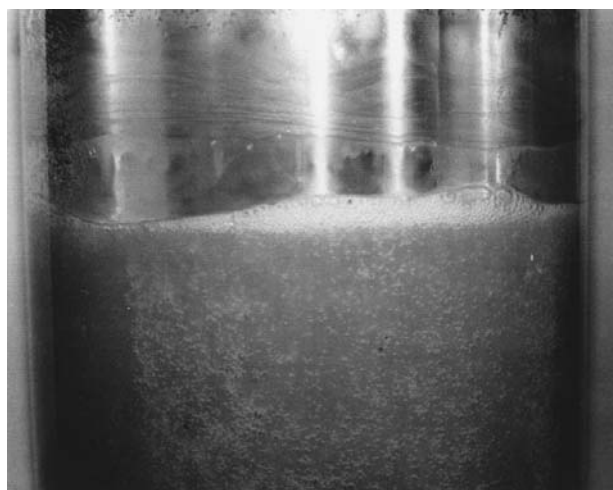
Figure 10. Mixing and mass transfer challenges in pullulan fermentation. The picture is taken when the agitator equipped with Ruston turbines is rotating at 500 rpm. The layer of fermentation broth adjacent to the fermenter wall remains stagnant with trapped air bubbles.
