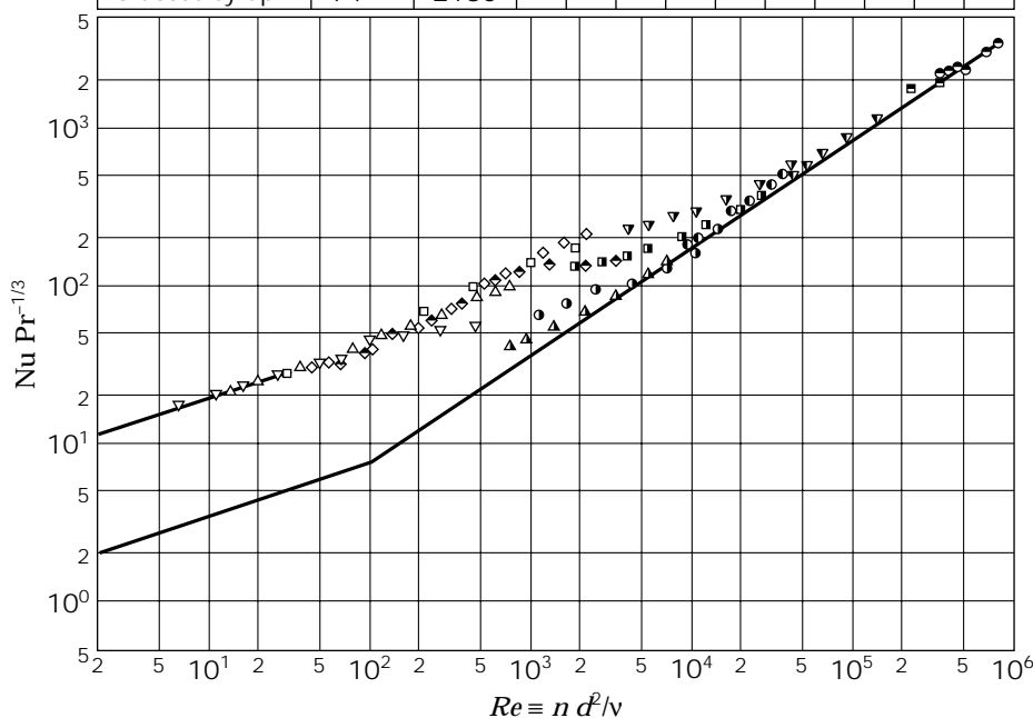
Figure 11. Enhancement of heat transfer at cooling in the laminar flow range ( Re < 10^3 ) by wiping the heat transfer surface. Measurements: anchor stirrer with four arms equipped with wipers. Solid curve: anchor stirrer with two arms, D/d = 1.02 (clearance \approx 2\% ). Source: From Ref. 20.
