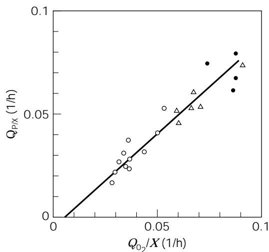
Figure 8. Dependence of the specific xanthan production rate on the specific oxygen uptake rate. Circles refer to runs in an STR at 15 L and 1,500 L, triangle correspond to bubble-column reactor; filled symbols denote no oxygen limitation.
