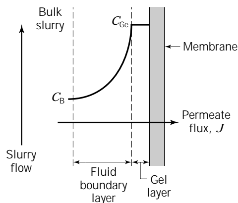
Figure 12. Steady-state solute concentration profile in ultrafiltration and microfiltration processes.
