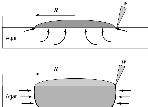
Figure 10. Schematic illustration of the difference between the growth modes bacterial (top) and fungi (bottom) colonies. Note that unicellular organisms ( bacteria ) do not penetrate into the agar layer as opposed to filamentous fungi. Arrows indicate directions of substrate diffusion across concentration gradients. R and w are, respectively, radius and width of the peripheral zone of the colony.
