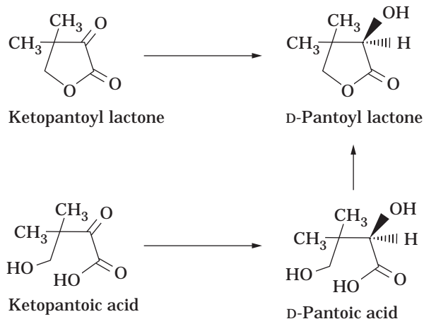
Figure 3. Production of D-pantoyl lactone.
