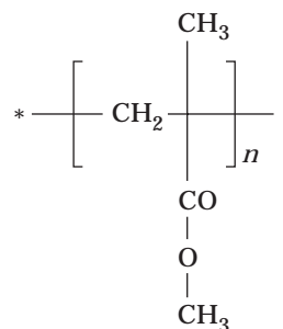
Poly(methylmethacrylate)
