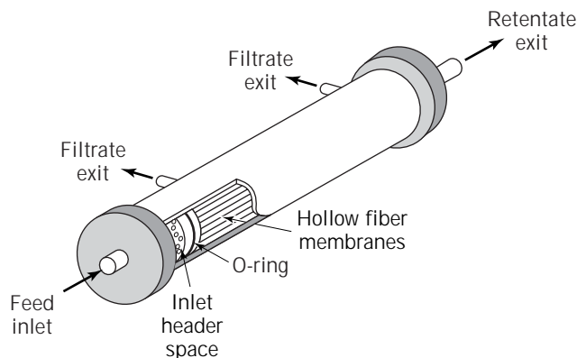
Figure 5. Schematic drawing of hollow-fiber module. Source: Adapted from Ref. 8. Courtesy of Marcel Dekker, Inc.
