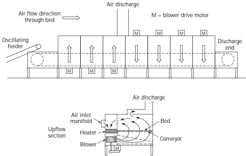
Figure 2. Conveyor dryer.
