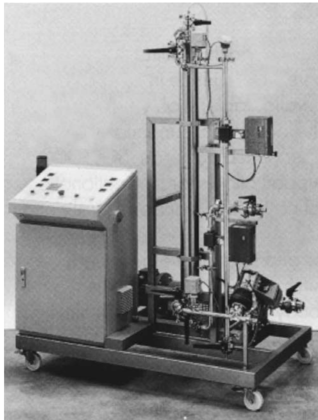
Figure 17. A small system with spiral-wound membrane modules. Source: Photo courtesy Millipore S.A., Molsheim, France.
