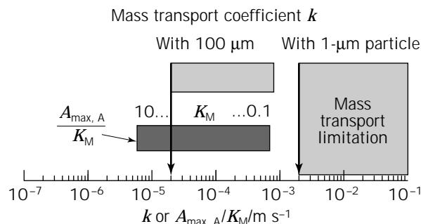
Figure 3. Influence of particle diameter on mass transport in comparison with enzymatic reaction.
