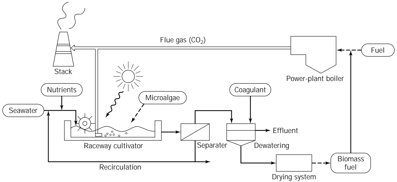
Figure 4. Conceptual system of CO 2 fixation by microalgae.
