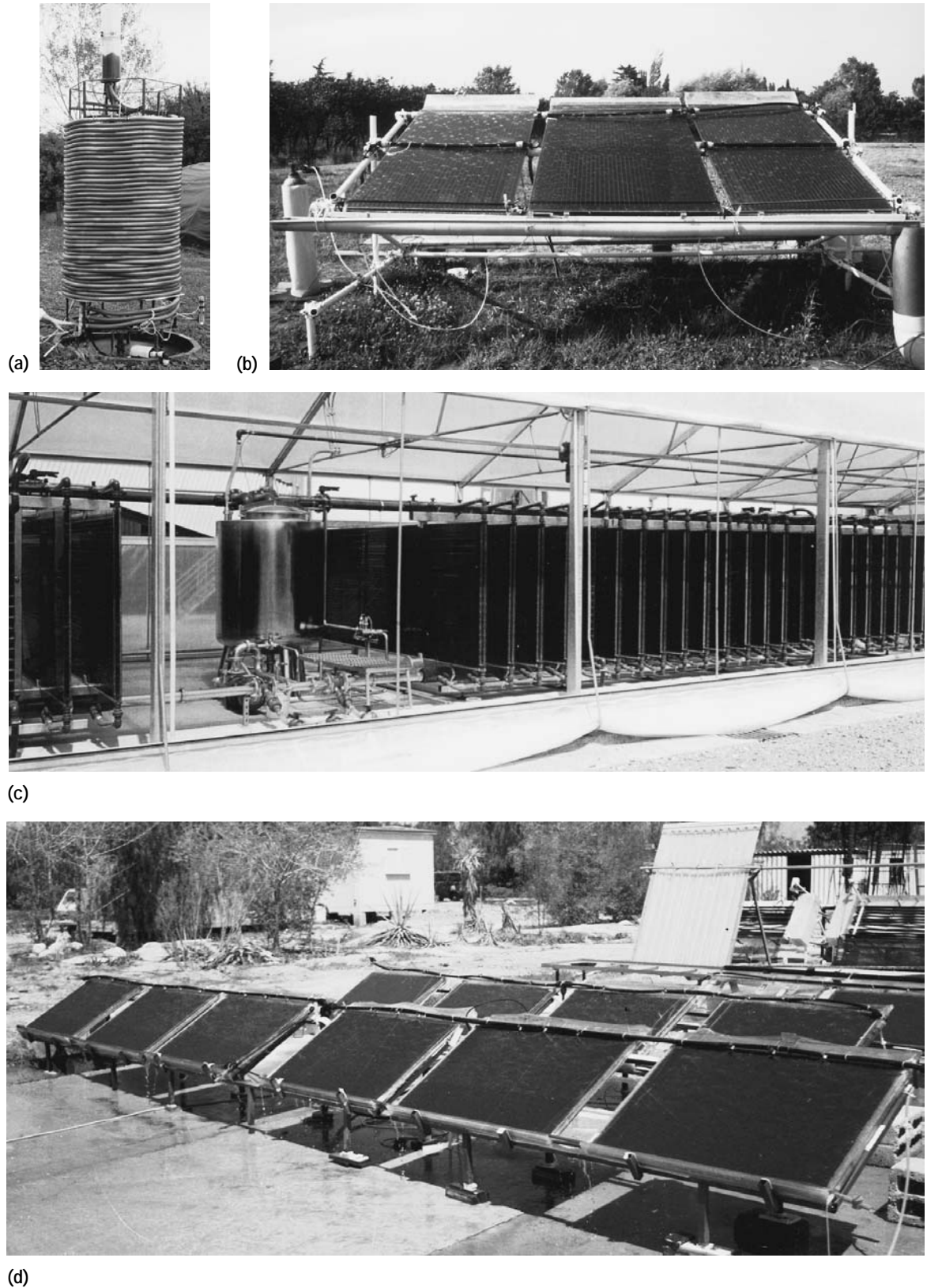
Figure 9. Biocoils and flat photobioreactors: (a) helical bubble-column reactor designed at the University of Florence, Italy (photograph by S. Pintus); (b) flat alveolar panels experimented with at the University of Florence, Italy (photograph by G. Chini Zittelli); (c) PBR system built by B. Braun Biotech Int., Germany (photograph courtesy of O. Pulz); (d) glass flat reactors experimented with at the Ben Gurion University of the Negev, Israel (photograph courtesy of A. Richmond).
