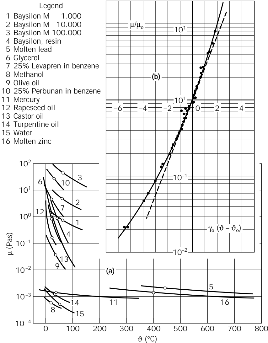
Figure 7. Temperature dependency of the viscosity \mu(\vartheta) and (b) its standard representation, which leads to the reference-invariant approximation of the material function. Data points on the curves in (a) mark the reference temperatures \vartheta_0 chosen. From (4, 11). Source: From Ref. 3, and Ref. 11.
