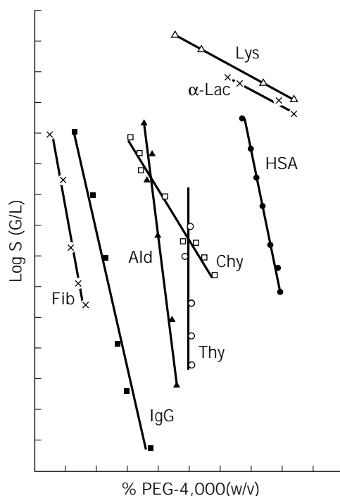
Figure 7. Solubility of various proteins in PEG-4,000. Measurements were made in 0.05 M potassium phosphate, pH 7.0, containing 0.1 M KCl. Human fibrinogen (×), human \gamma -globulin (■), lysozyme ( \Delta ), \alpha -lactalbumin (+), chymotrypsin ( \square ), aldolase ( \blacktriangle ), thyroglobulin ( \circ ), human serum albumin ( \bullet ).
