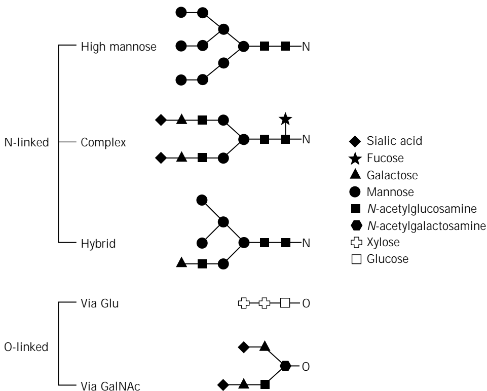
Figure 1. Common oligosaccharide structures found on glycoproteins.
