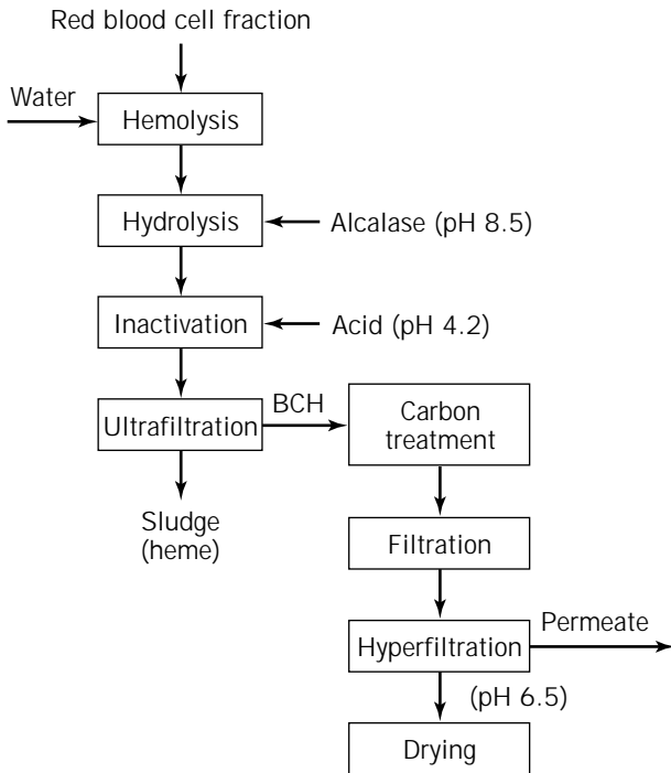
Figure 23. Flowchart for production of blood cell hydrolysate.
