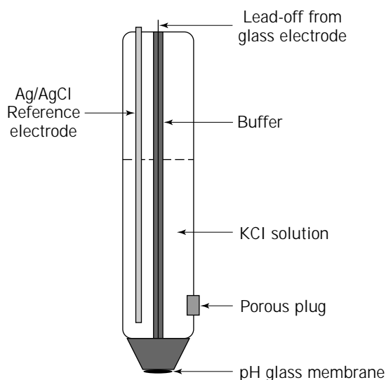
Figure 4. pH electrode.
