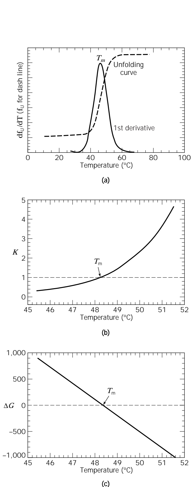
Figure 2. Methods for determining T_m value from protein unfolding curves (the plots were based on data shown in Figure 1) A) f_U (% protein unfolded) and df_U/dT versus T ; B) K versus T ; C) \Delta G versus T . (a) First derivative of the fraction of unfolded protein as a function of temperature. (b) Equilibrium constant versus temperature. (c) Gibbs free energy versus temperature.
