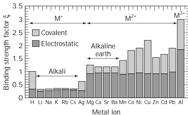
Figure 4. Binding-strength parameters for different metals.
