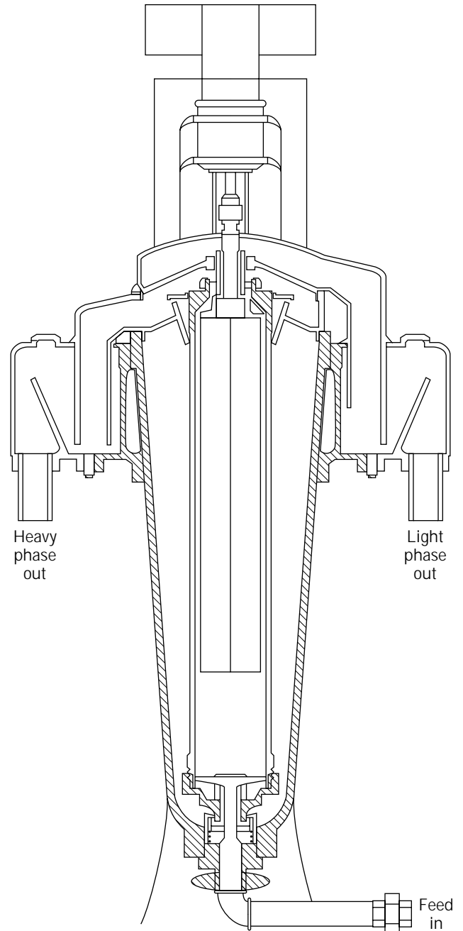
Figure 6. Tubular bowl centrifuge, vertical cut.
