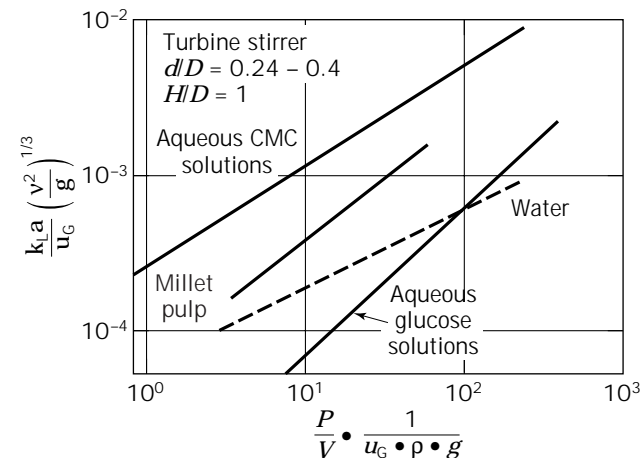
Figure 14. Sorption characteristics for millet pulp, glucose solutions, and CMC solutions.
