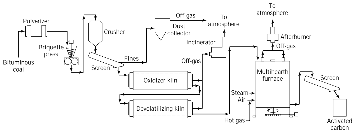
Figure 1. Thermal activation of bituminous coal.
