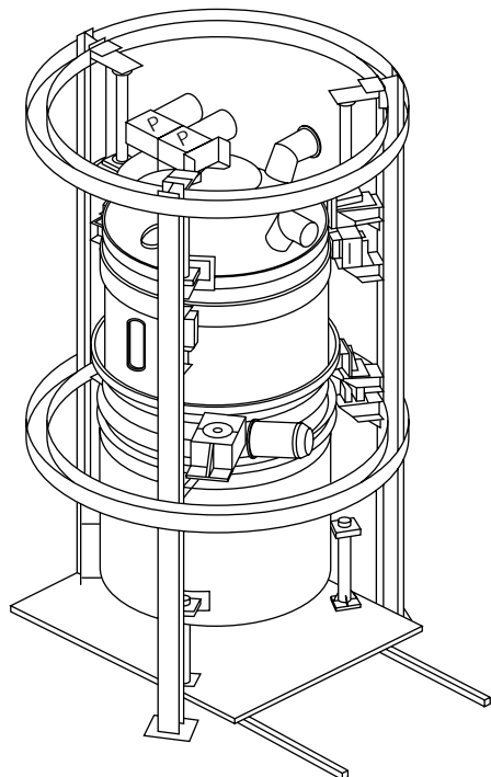
Figure 12. A 200-kg SSF pilot bioreactor.
