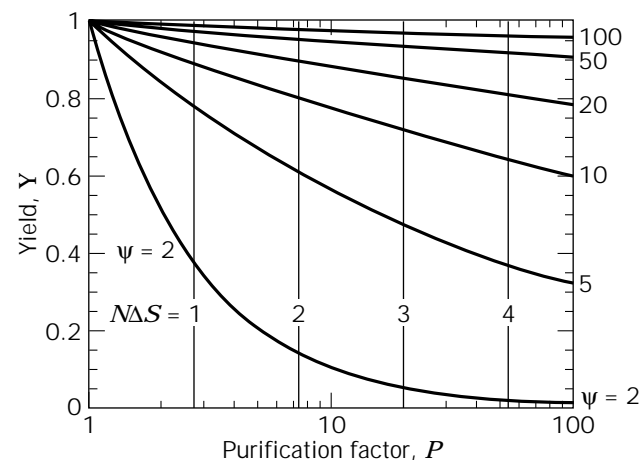
Figure 16. Optimization diagram for product in the retentate. The process follows a constant selectivity ( \psi ) curve starting at a fractional yield Y = 1 and can be operated up to a maximum N\Delta S , which depends on the experimental J\Delta S value and the ratio of membrane area ( A ), process time ( t ), and retentate volume ( V ). Source: Adapted from R. van Reis and S. Saksena (52). With kind permission of Elsevier Science-NL, Amsterdam, The Netherlands.
