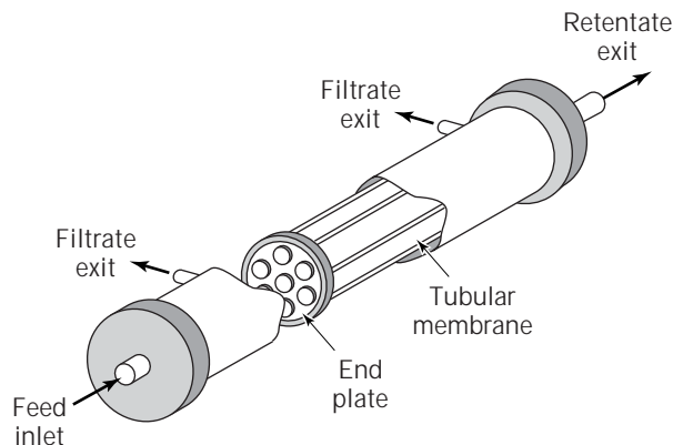
Figure 6. Schematic drawing of tubular module. Source: Adapted from Ref. 8. Courtesy of Marcel Dekker, Inc.
