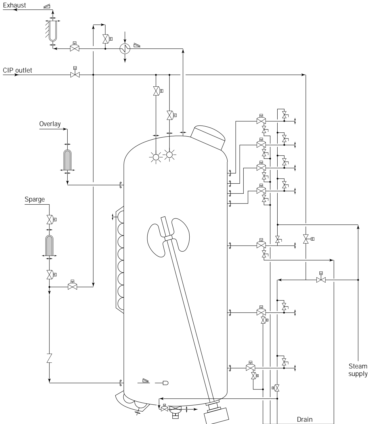
Figure 18. Simplified CIP piping diagram.
