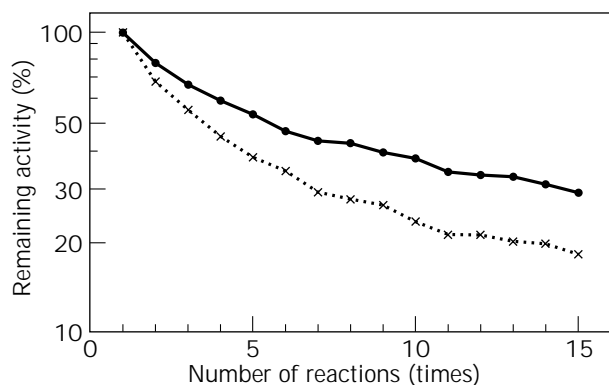
Figure 8. Stability of the immobilized DCase on repeated batch reactions. Repeated batch reactions were carried out using the immobilized mutant DCase from KNK404M (circles) and the native enzyme (asterisks).
