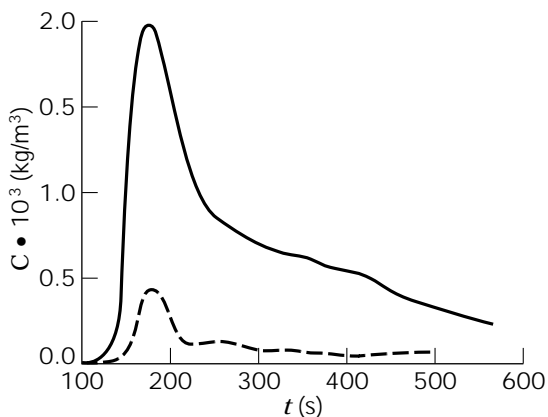
Figure 17. Pulse response at the exit of a tube equipped with the static mixer in Figure 1c, - - - - = without static mixer; — = with static mixer.
