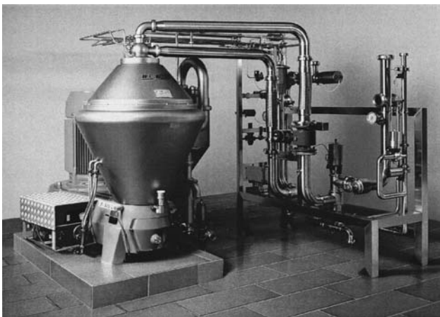
Figure 3. Solids-ejecting disk bowl centrifuge of production size. Capacity in breweries up to 75 m 3 /h. Type BREW 2000. The height of the separator is 2.2 m. Source: Courtesy of Alfa-Laval Separation AB.
