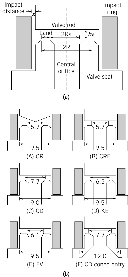
Figure 4. (a) Schematic diagram of a typical valve unit. (b) Schematic diagram of valve units used: (A) CR, cell rupture with coned valve rod; (B) CRF, cell rupture with flat valve rod; (C) CD, cell disruption; (D) KE, knife edge; (E) FV, flat valve unit; (F) CD-type unit with coned entry—dimensions in millimeters. Land distances ( R - R_0 ) are for CRF, 0.7 mm; CD, 0.5 mm; KE, 0.1 mm; FV, 1.5 mm. Source: Reprinted by permission of Elsevier Science Inc. from Ref. 35.
