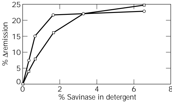
Figure 8. Launder-O-meter data of Savinase 6.0 T. Test system: EMPA 117; 4 g/L European powder detergent: —□—, 40 °C for 47 min; —○—, 60 °C for 40 min.
