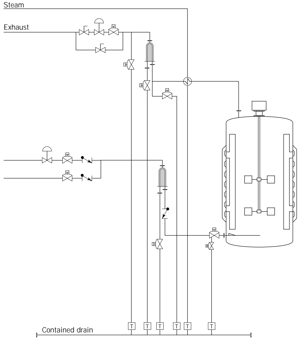
Figure 12. Simplified piping diagram illustrating air inlet and outlet systems.
