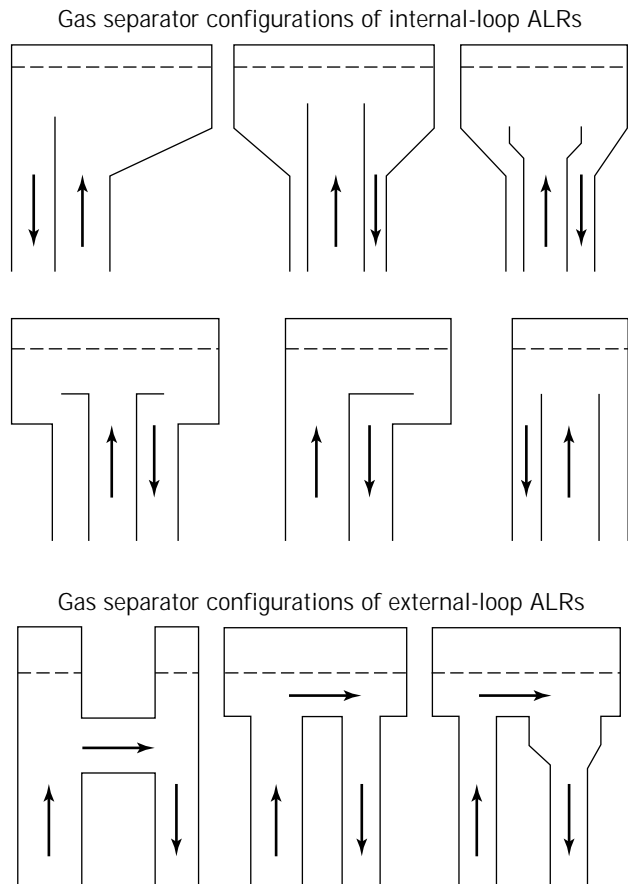
Figure 2. Different types of gas separators.
