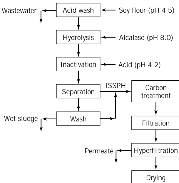
Figure 24. Flowchart for production of isoelectric soluble soy protein hydrolysate (ISSPH).
