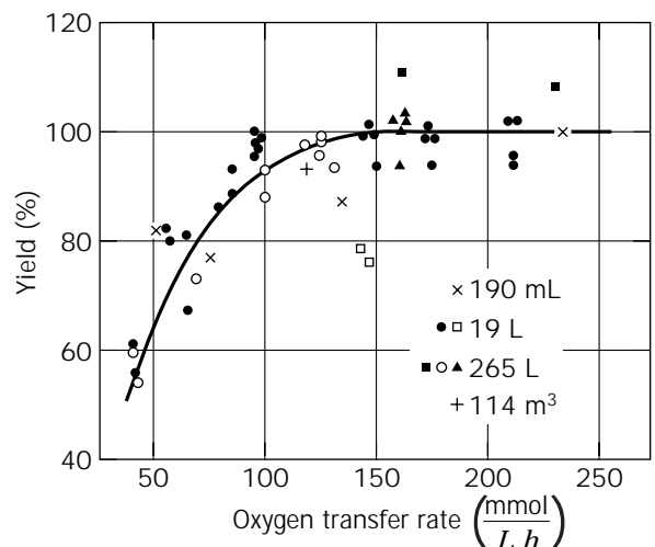
Figure 19. Scale-up of fermentation of baker's yeast based on oxygen transfer rate (sulfite oxidation).
