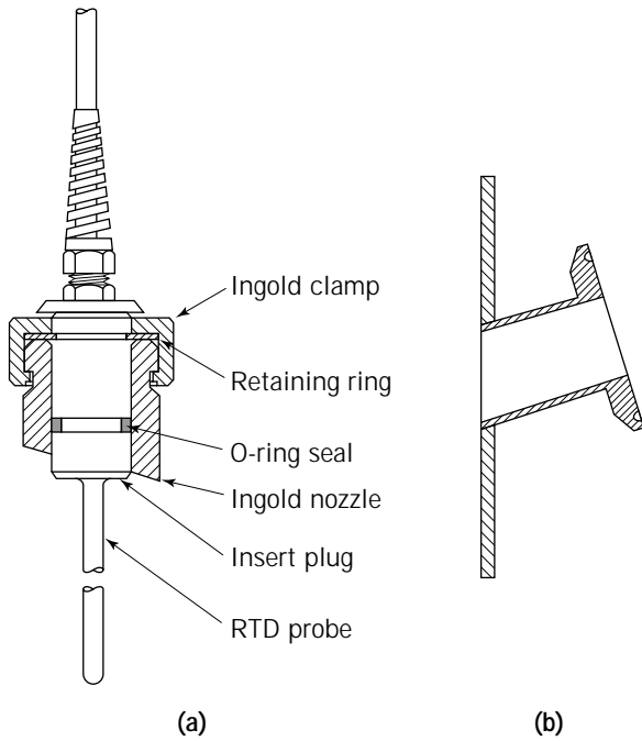
Figure 6. Ingold and sanitary clamp fittings.
