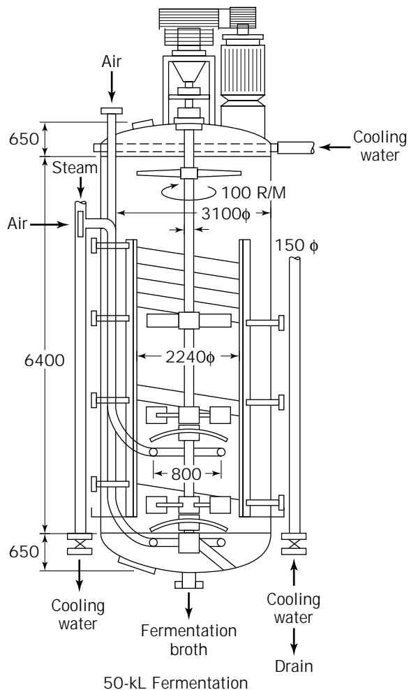
Figure 7. Example of an industrial fermenter. R/M, revolutions per minute; \phi , diameter; all distances in millimeters. Source: From Y. Su and K. Yamada, Bull. Agric. Chem. , 1960, cited in Ref. 17.
