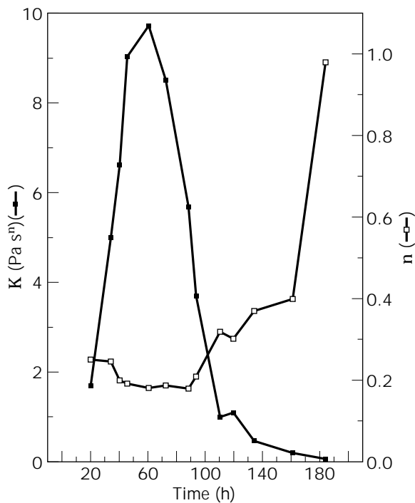
Figure 9. Variation of consistency index, K , and flow behavior index, n , of S. rimosus industrial strain culture as a function of time of the fermentation.
