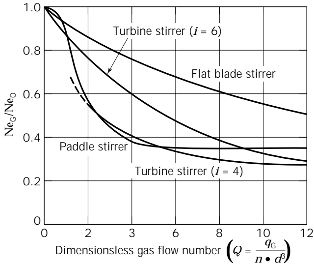
Figure 4. Power input of several types of stirrer in Newtonian fluids, dependent on the gas throughput.
