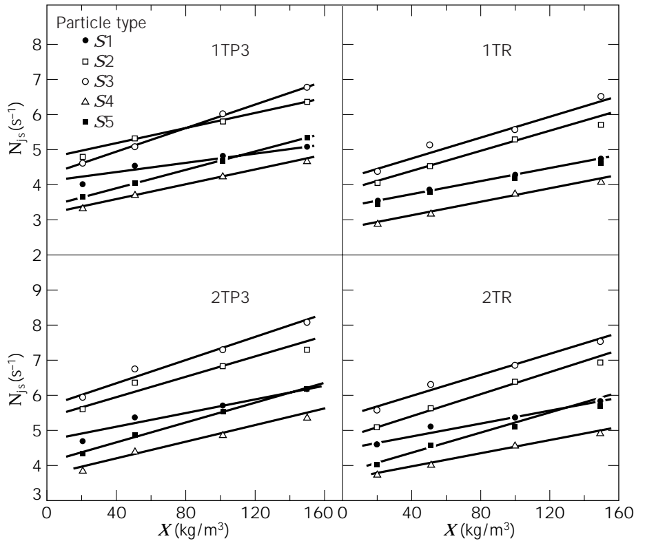
Figure 5. Effect of solid concentration on complete suspension speed for standard and modified Rushton turbines, positioned singly or doubly on the same shaft. S1–S5, particle types (see Table 2). (Source: From Ref. 20, with permission.)
