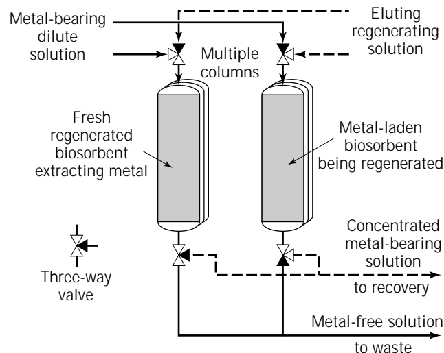
Figure 1. Schematic flowchart of a continuous-flow column biosorption process.
