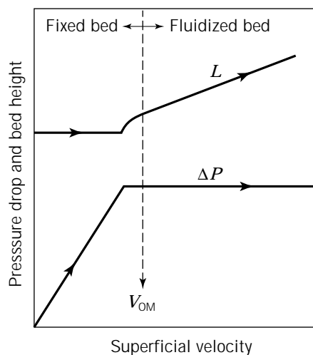
Figure 1. Illustration of the basic concept of fluidization. Variation of the pressure drop ( \Delta P ) and the height of the solid particles in a bed ( L ), with increasing fluid superficial velocity. V_{0M} , minimum fluidization velocity.
