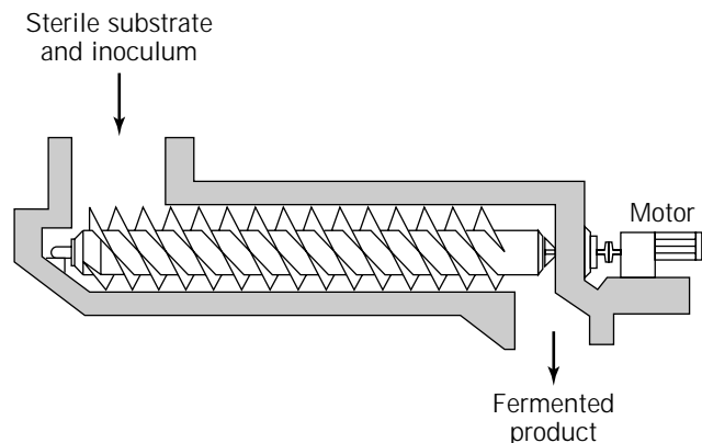
Figure 7. Screw fermentor for continuous fermentation.
