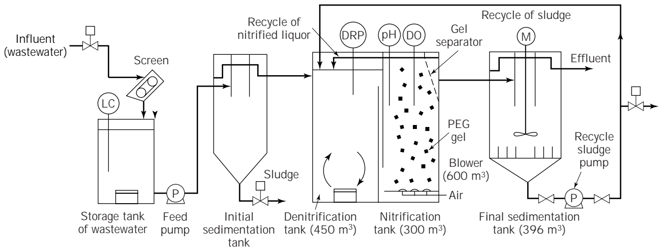
Figure 4. Schematic diagram of wastewater treatment plant with a capacity of 2,250 m 3 /day (max, 3,000 m 3 /day). DO = dissolved oxygen electrode; ORP = oxidation–reduction potential; pH = pH electrode; LC = level control; P = pump; M = mixer.
