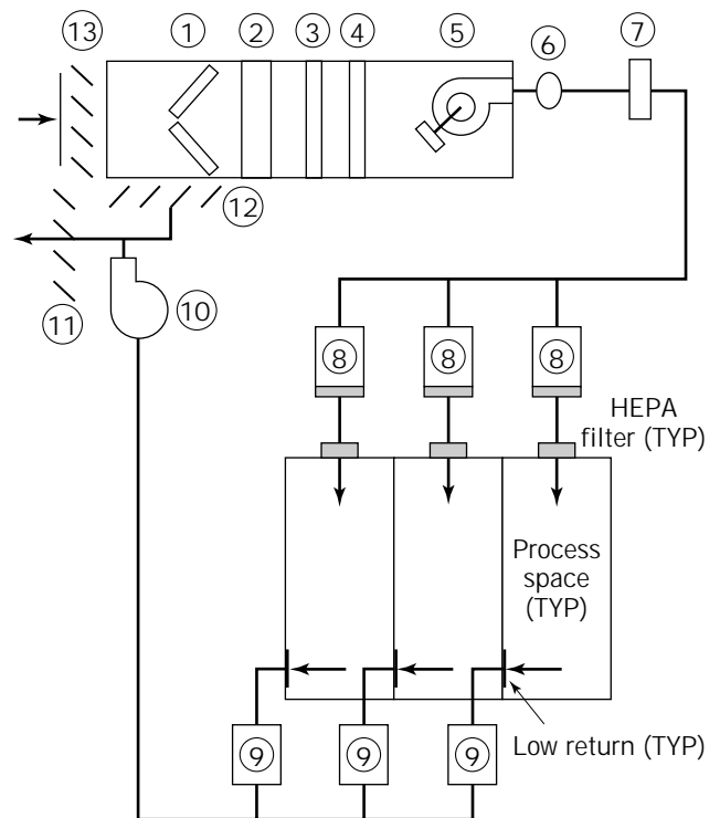
Figure 3. Airflow diagram: 1, 35% filters; 2, 85% filters; 3, pre-heat coil; 4, cooling coil; 5, fan section; 6, humidifier; 7, air monitoring device; 8, constant volume reheat box; 9, constant volume box; 10, return fan; 11, relief air damper; 12, return air damper; 13, outdoor air damper.
